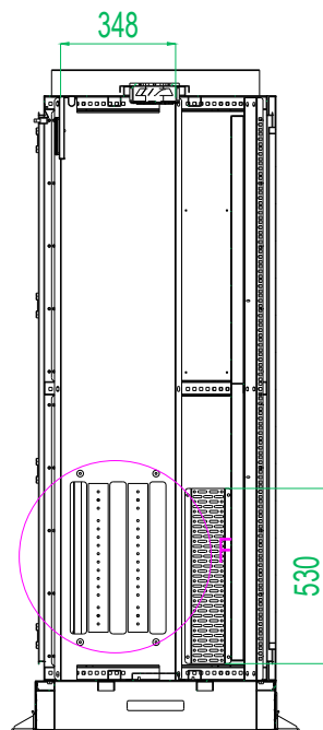
SECTION F-F
