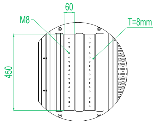
DIMENSION F 1: 14
