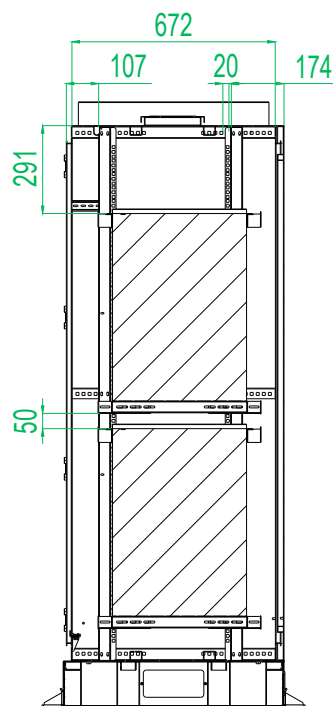
SECTION F-F
